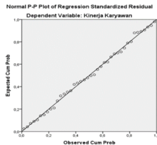
Hasil Uji Normalitas Grafik Normal Probability Plot
