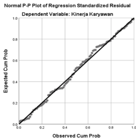
Gambar 1. Hasil Uji Normal Probability Plots
