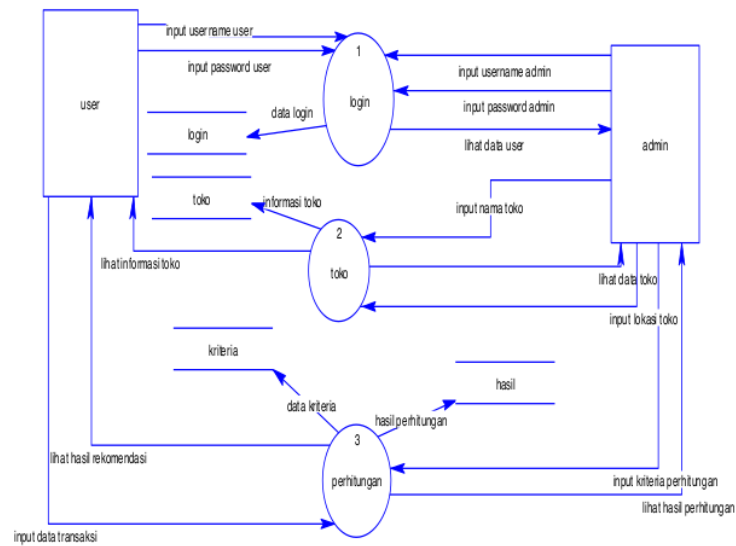
Gambar 2.3 DFD Level 0
