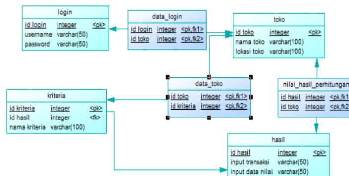
Gambar 2.5 PDM
