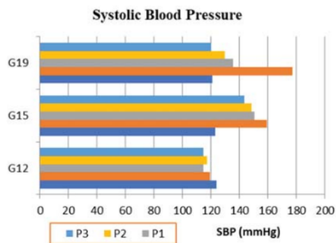
FIGURE 1. Systolic Blood Pressure Measurements in Preeclampsia Rats Pregnant Model Given Different Doses of Pravastatin. The mean systolic blood pressure of pregnant rats model of preeclampsia was measured at the 12th, 15th, and 19th gestation. K(-) is a group of normal pregnant rats, K(+) is a pregnant rat model of preeclampsia, P1, P2, and P3 are rats of a preeclampsia model given pravastatin with doses of 2 mg/day, 4 mg/day and 8 mg/day.
