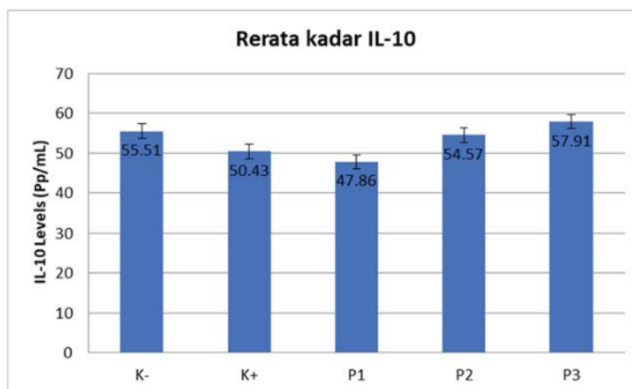
FIGURE 4. Effect of pravastatin on IL-10 serum levels in preeclampsia model rats. The one-way ANOVA test shows a significant difference with p=0.001<\alpha . LSD test result shows that there is a significant difference between the two groups, which showed p=0.000 . The statistical test shows that 8 mg/day is the optimum dose and a stronger positive correlation in increasing IL-10 levels in preeclampsia model Wistar rats ( r=0.882 ; correlation is significant at the 0.01 level).
