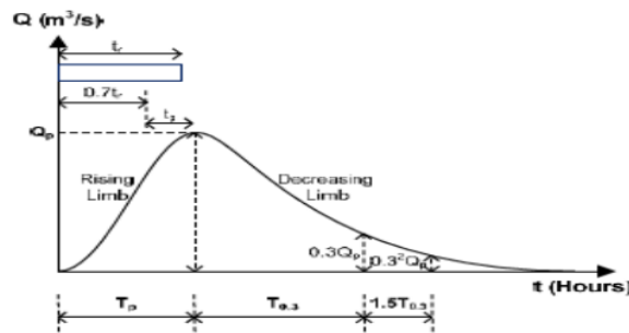
Figure 2. Scheme of Synthetic Unit Hydrograph of Nakayasu
