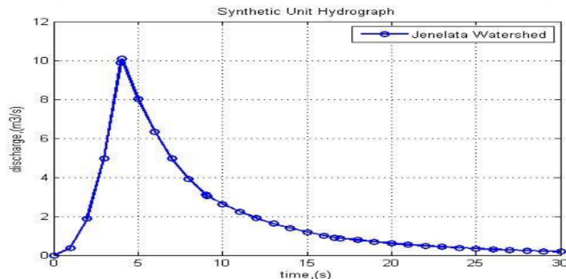
Figure 3. Nakayasu synthetic unit hydrograph of Jenelata Watershed
