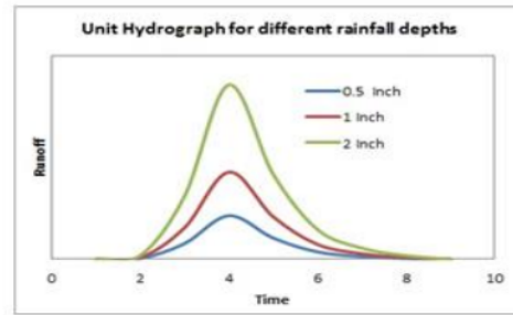
Figure 1. Unit hydrograph for different rainfall depth
