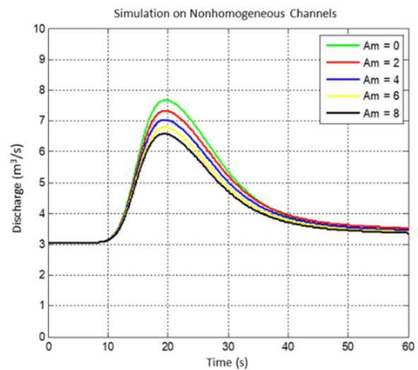
Figure 6. The Appearance Variety Top Discharge as a Result of a Variety of the Width of the Pocket of Flood
