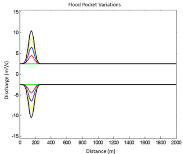
Figure 5. Profile of Pocket of Flood with Varies Width among of A_m = 0, A_m = 2, A_m = 4, A_m = 6, and A_m = 8
