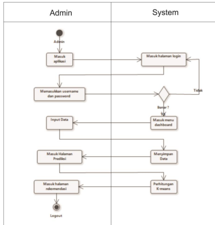
Gambar 3.2 Activity diagram
