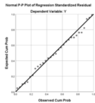
Gambar 1.1 Normal Probability Plot
