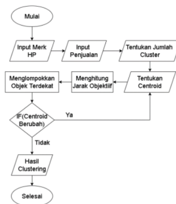
Gambar 1. Flowchart
