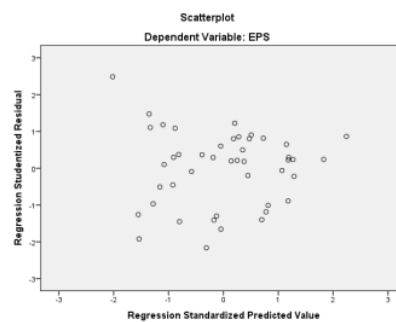
Gambar 1. Heteroscedasticity Test
