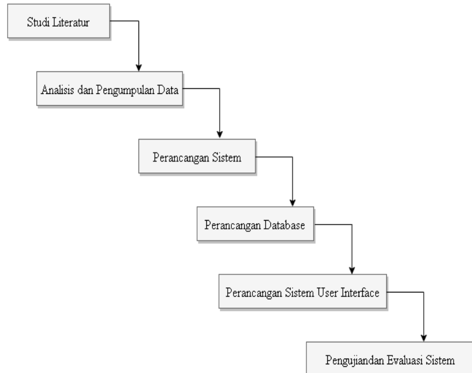
Gambar 1.1 Diagram Waterfall
