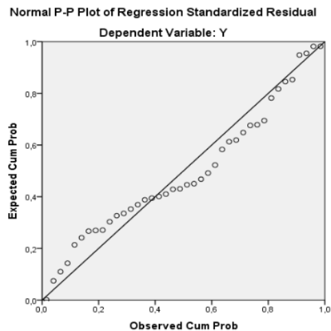
Gambar 1. Uji Normalitas Probability Plots
