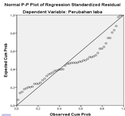
Gambar 1. Hasil Uji Normalitas Probability Plots
