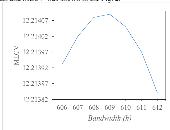
FIGURE 2. Plot between bandwidth and MLCV
