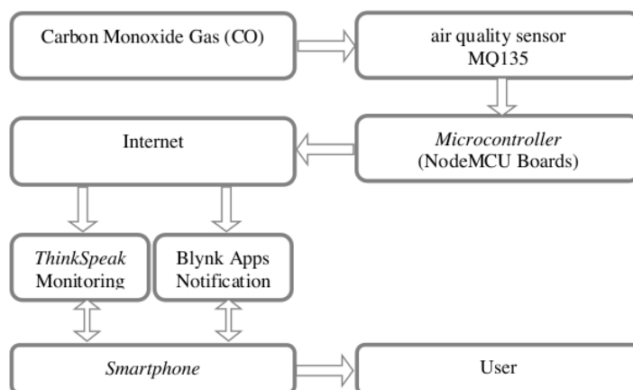
Figure 2. BLOCK DIAGRAM OF MONOXIDE CARBON DETECTION SYSTEM
