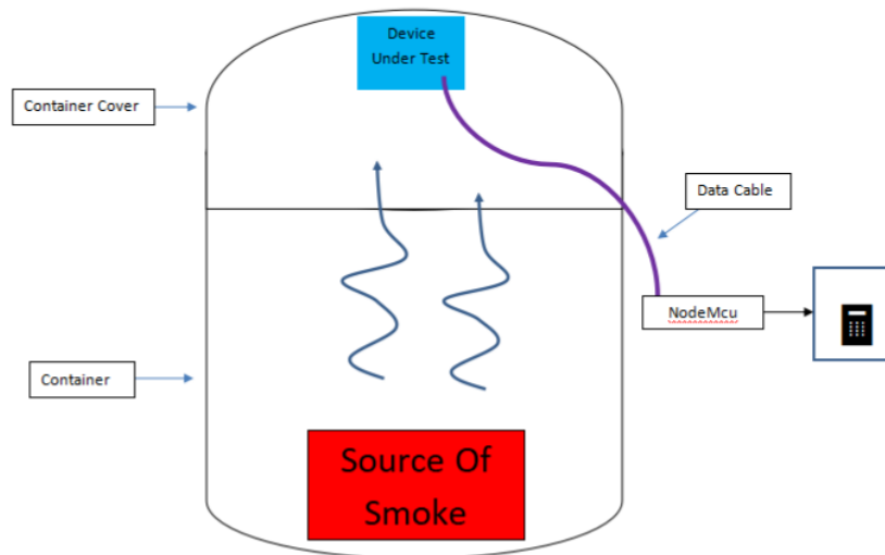
Figure 4. MONOXIDE CARBON DETECTION SYSTEM TESTING SCHEME
