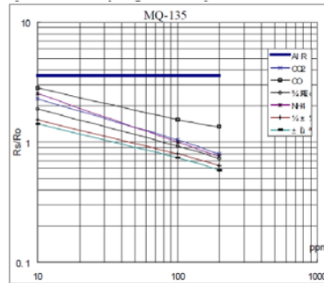
Figure 3. MQ135 SENSITIVITY CHARACTERISTICS
