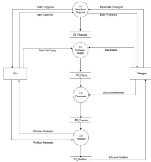
Gambar 2 DFD Level 1
