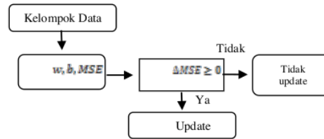
Gambar 2 Proses Training ELM terintegrasi (Mahdiyah, 2017)
