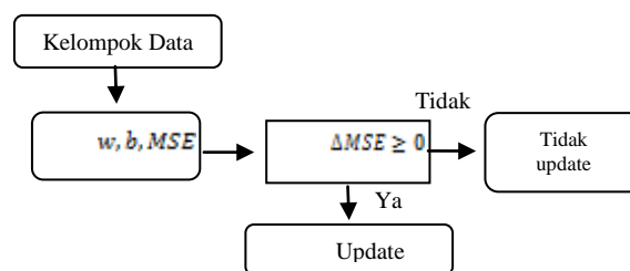
Gambar 2 Proses Training ELM terintegrasi (Mahdiyah, 2017)
