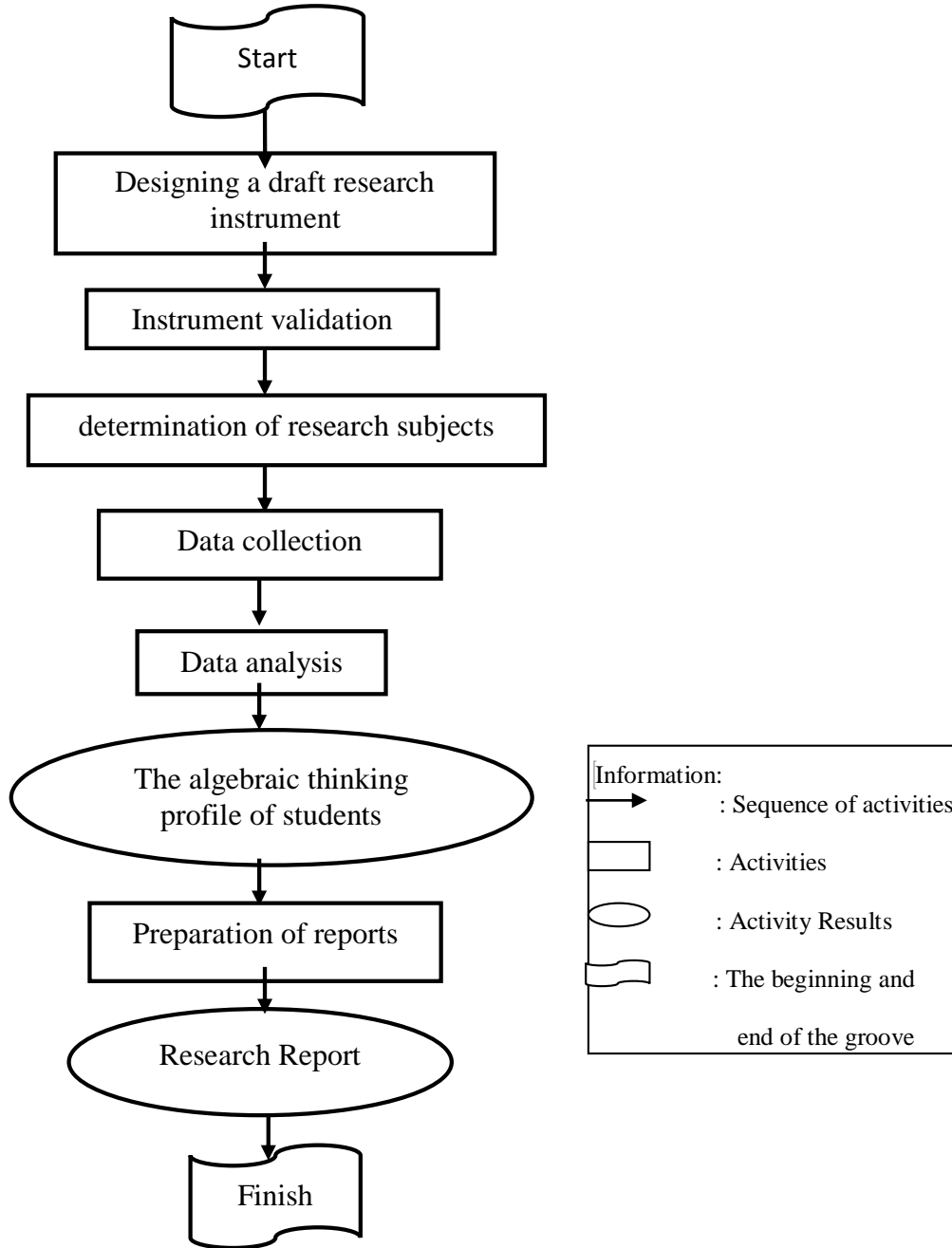
Figure 1. Research Flowchart
