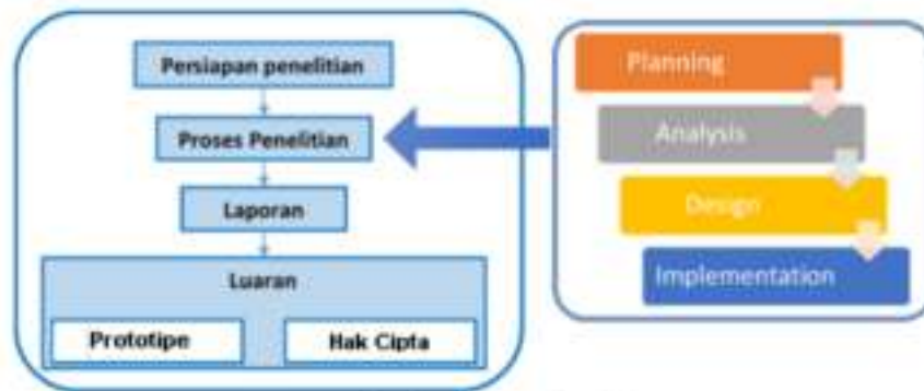
Gambar 1 Bagan Penelitian
