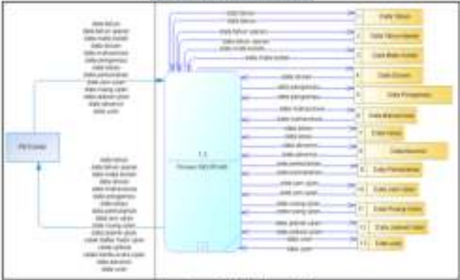
Gambar 4. DFD Level I
