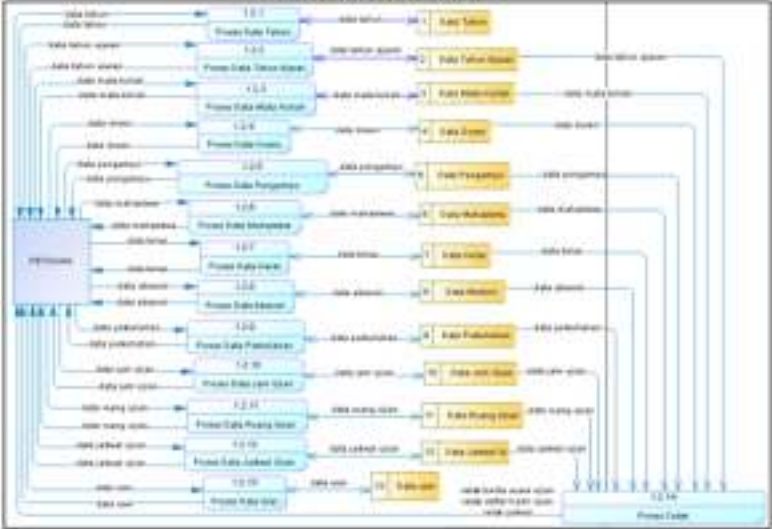
Gambar 5. DFD Level 2
