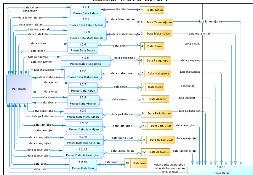
Gambar 5. DFD Level 2
