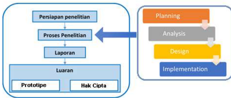
Gambar 1 Bagan Penelitian
