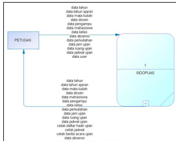
Gambar 3. DFD Level 0
