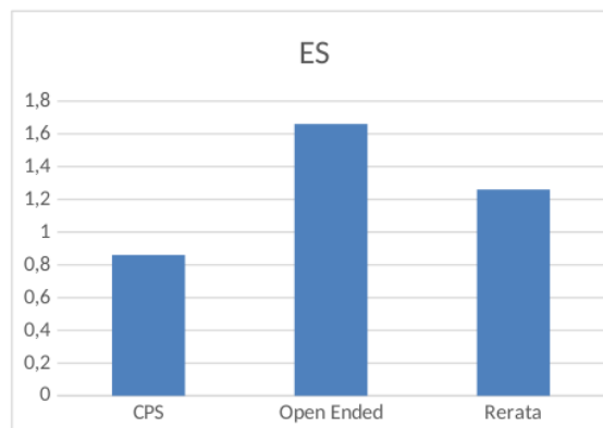
Gambar 1. Diagram nilai rata-rata effect size
