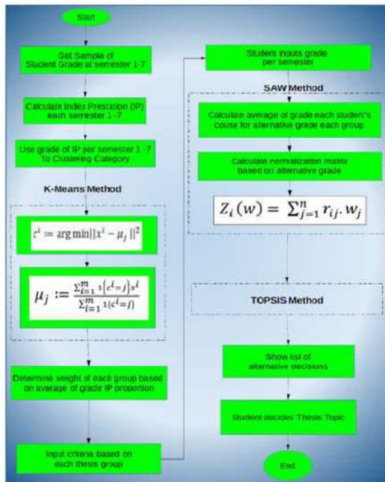
Fig. 2. Overview of Decision Support System Design
