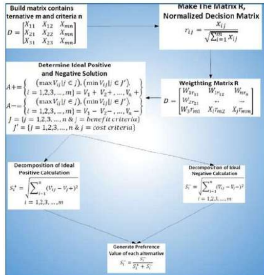
Fig. 3. Flow of TOPSIS Calculation
