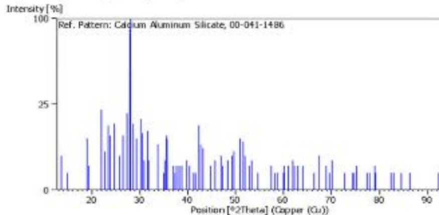
Gambar 2.3 Identifikasi fasa anorthite ( \text{CaAl}_2\text{Si}_2\text{O}_8 )
