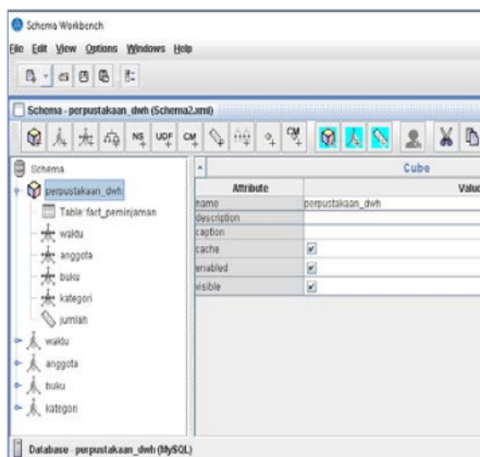
Gambar 11. Pentaho Schema Workbench
