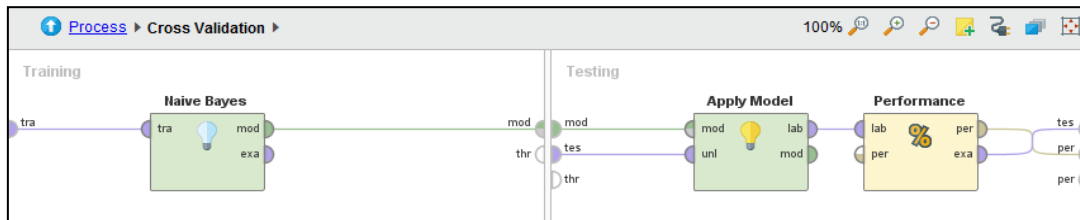
Fig. 3 Sub-process of Cross Validation in RapidMiner
