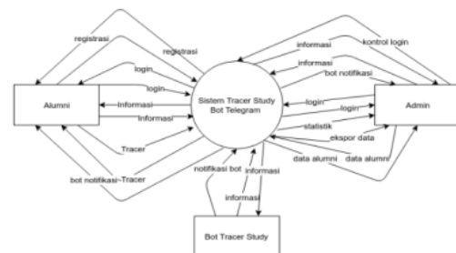
Figure 3. Level 0 DFD
