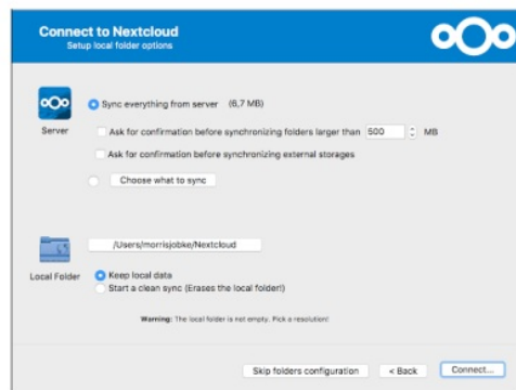
Gambar 8. Connection Nextcloud
