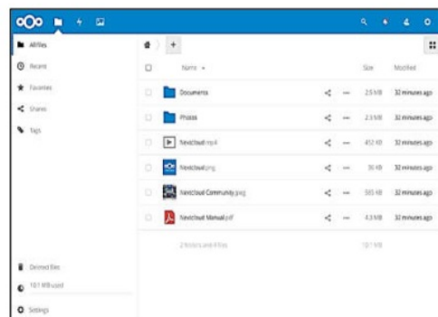
Gambar 7. Menu Nextcloud
