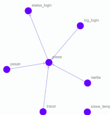
Figure 4. Database Relation
