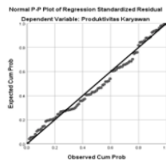
Gambar 4.3 Hasil Uji Normalitas Probability Plot
