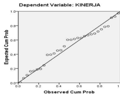
Gambar 6 Hasil Uji Normal Probability Plots
