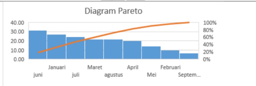
Gambar 1.2 Diagram Pareto
