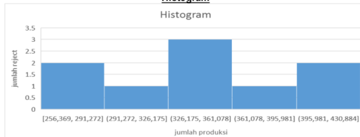
Gambar 1.1 Histogram
