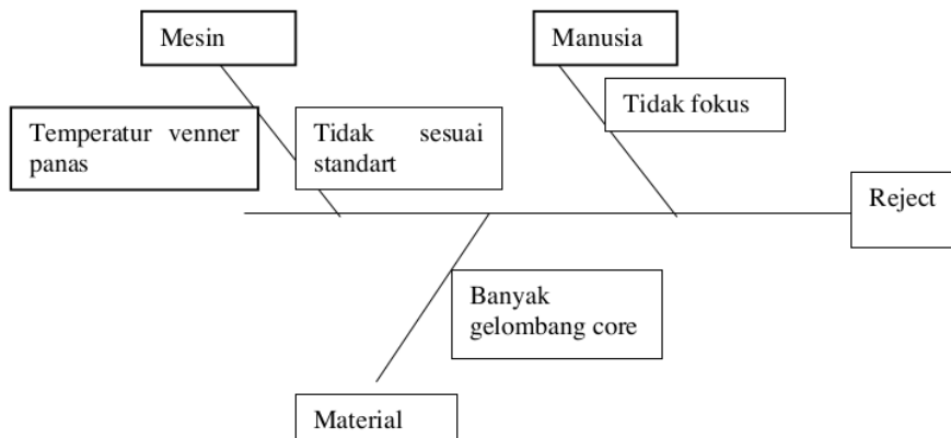
Gambar 1.4 Diagram Fishbone
