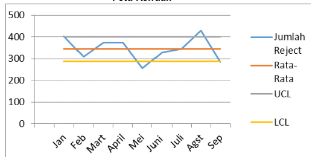
Gambar 1.3 Peta Kendali
